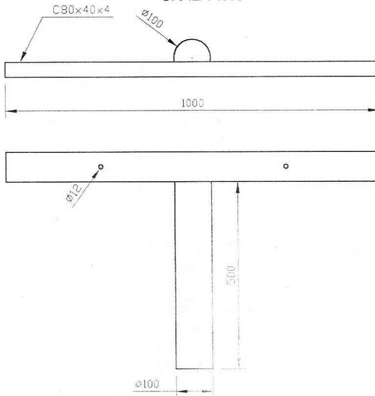
WN-1000 SKALA 1:10
