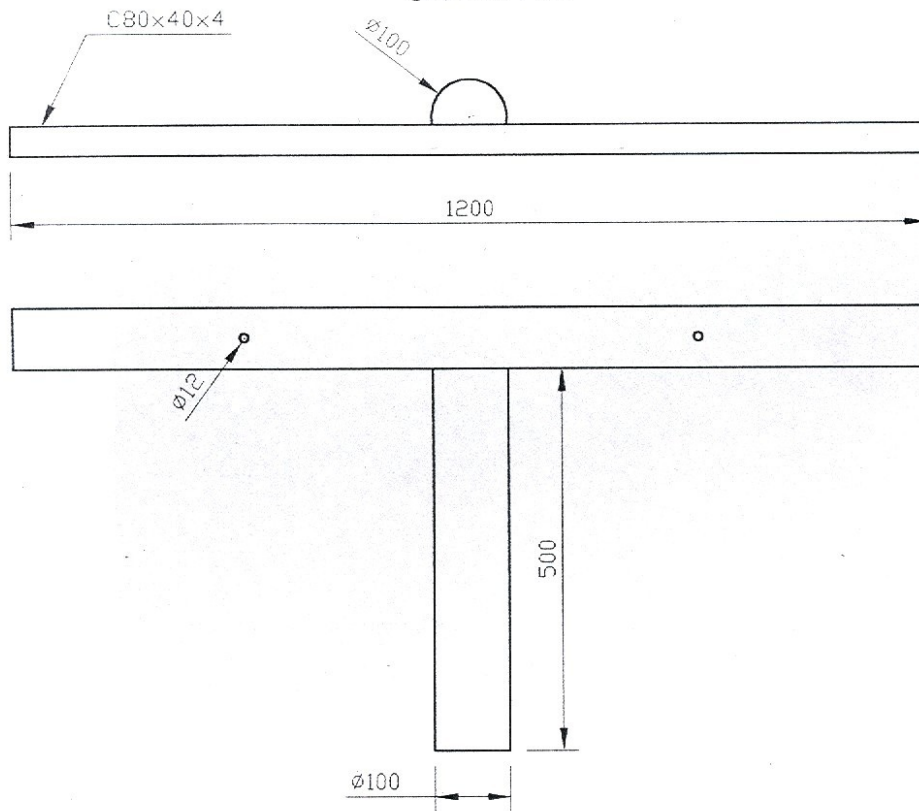
WN-1200 SKALA 1:10
